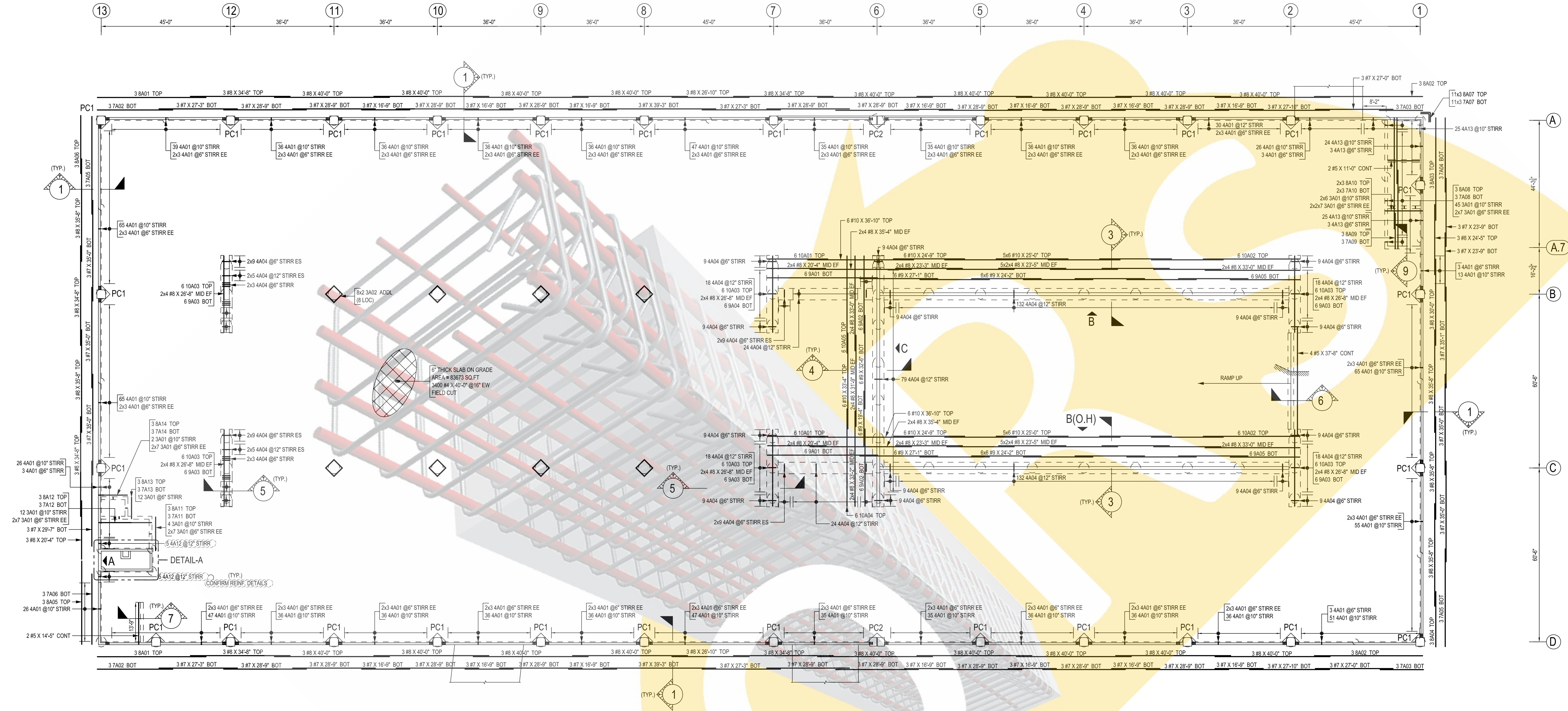
FOUNDATION REBAR LAYOUT SCALE: 1/16"=1'-0" SDR: S101
